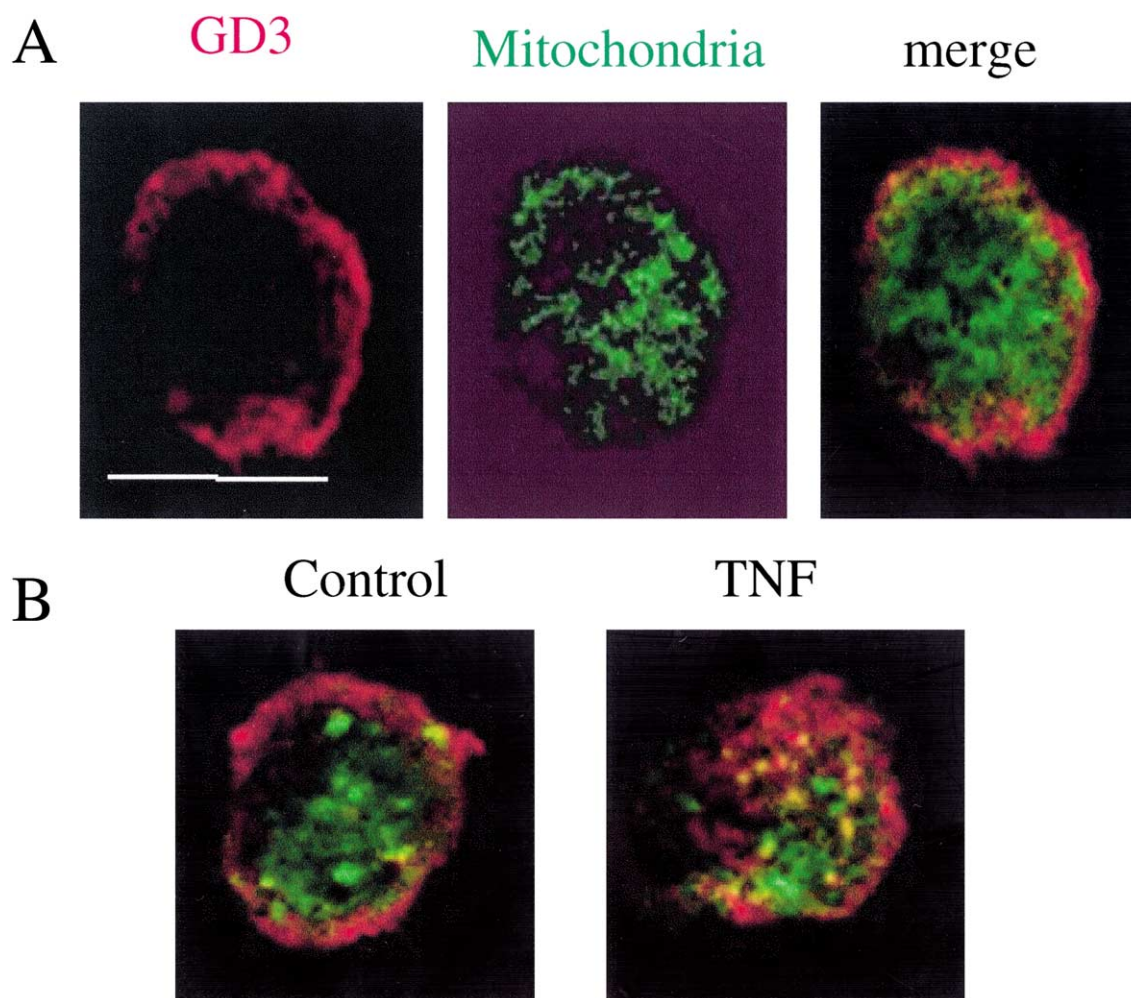
Fig. 5. Cellular distribution of GD3 by TNF. A: HT-29 cells were immunostained with antibodies anti-GD3 and anti-mitochondrial, followed by appropriate secondary antibodies. Merged images of red (GD3) and green (mitochondria) fluorescence were collected in a confocal microscope. B: HT-29 cells were treated with TNF (280 ng/ml), for 8 h and then cells were fixed and immunostained for GD3 and mitochondria localization. At least 100 cells per condition were examined. Less than 10% of control cells displayed merged fluorescence, while those exhibiting co-localization by TNF were observed in more than 85% of the cells examined. Representative images of four independent experiments showing similar results. Bar is 10 \mu m.
