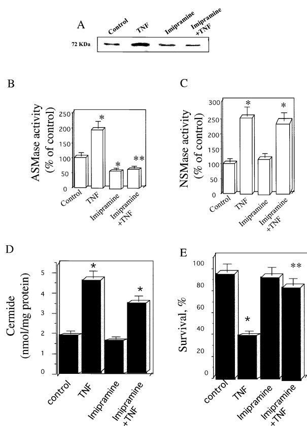
Fig. 2. Involvement of ASMase in TNF-mediated cell death. HT-29 cells were treated with TNF (280 ng/ml) for 12 h in the absence or presence of imipramine (20 \mu M). Cell extracts were isolated and resolved by SDS-PAGE followed by incubation with antiserum anti-ASMase (A). Parallel cell extract aliquots were used for ASMase (B) or NSMase (C) activity determined from [ N -methyl- 14 C]sphingomyelin (56.6 mCi/mmol) hydrolysis. Cells were then treated with chloroform:methanol and lipid extracts used for ceramide determination by HPLC (D). Survival of HT-29 cells after TNF (280 ng/ml) for 20 h with or without imipramine treatment was determined by MTT assay (E). Results are the mean \pm S.D. of five independent experiments. * P < 0.05 vs. control; ** P < 0.05 vs. TNF.
